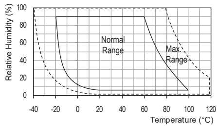
Figure 4. Operating Conditions
